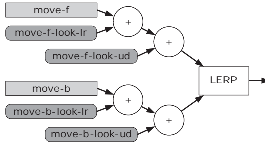
Figure II.56. Blend tree corresponding to the example state “move-b-to-f.”
