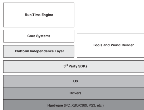
Figure 1.32. Standalone tools architecture.
