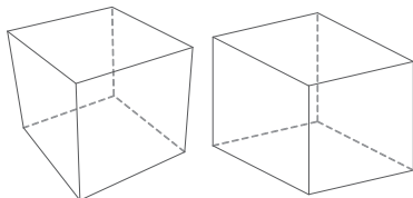
Figure 10.31. A cube rendered using a perspective projection (on the left) and an orthographic projection (on the right).
