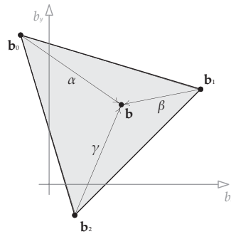
Figure 11.36. Various barycentric coordinates within a triangle.
