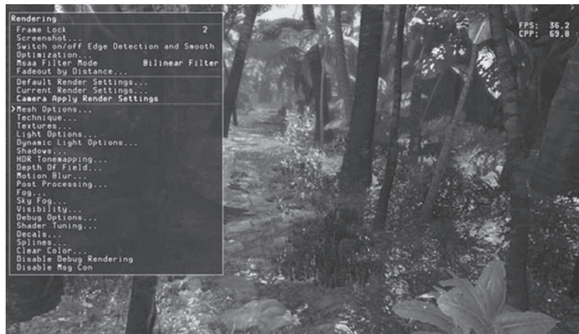
Figure 9.6. Rendering submenu.
