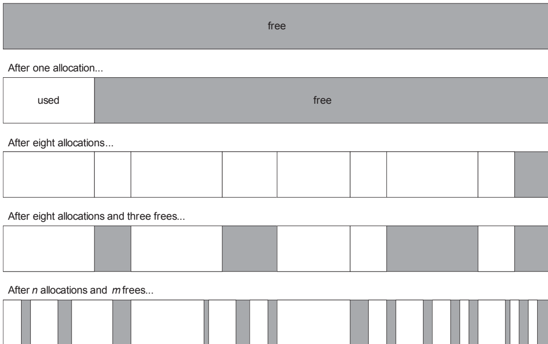
Figure 5.3. Memory fragmentation.
