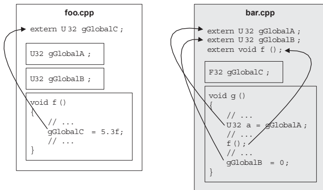
Figure 3.7. Unresolved external references in two translation units.
