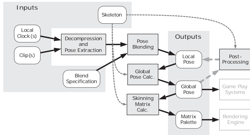
Figure II.44. A typical animation pipeline.
