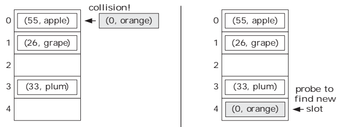
Figure 5.II. A closed hash table.
