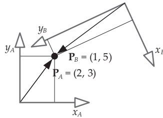
Figure 4.16. Position vectors for the point P relative to different coordinate axes.
