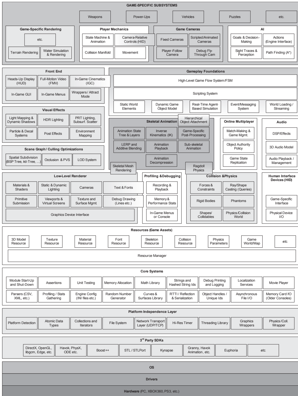
Figure 1.II. Runtime game engine architecture.
