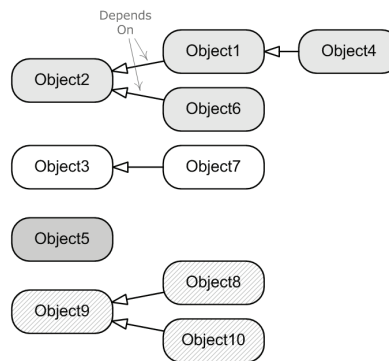
Figure 14.14. Inter-object update order dependencies can be viewed as a forest of dependency trees.
