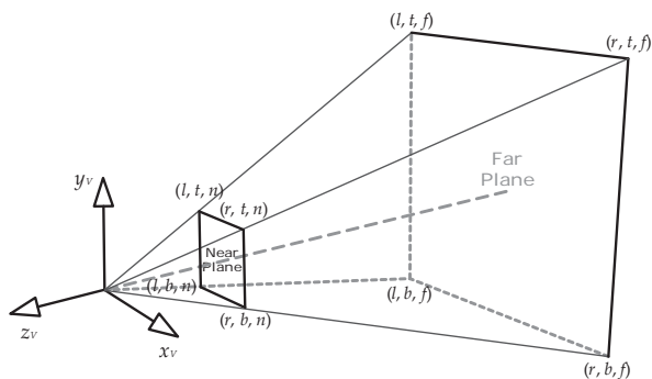
Figure 10.32. A perspective view volume (frustum).
