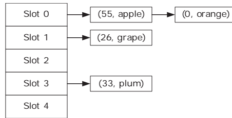
Figure 5.I0. An open hash table.
