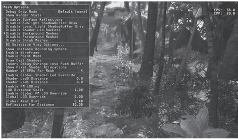
Figure 9.7. Mesh options subsubmenu.
