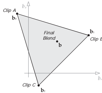
Figure II.35. Two-dimensional animation blending between three animation clips.
