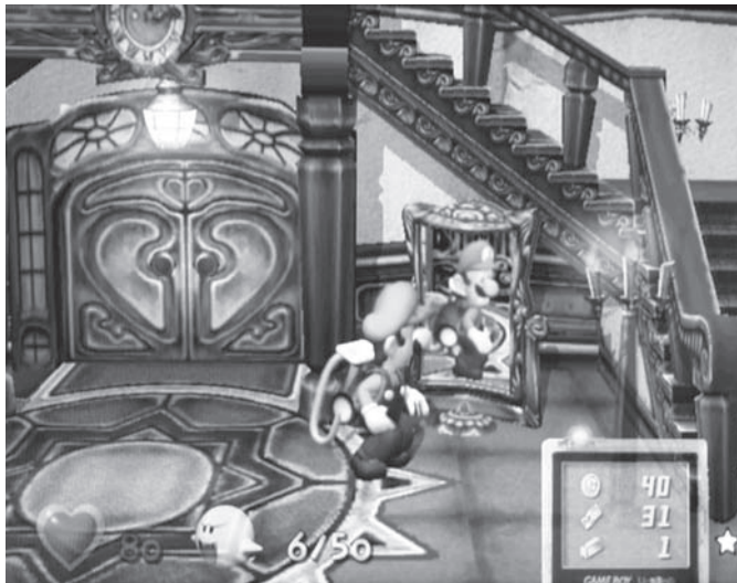
Figure 10.54. Mirror reflections in Luigi's Mansion implemented by rendering the scene to a texture that is subsequently applied to the mirror’s surface.
