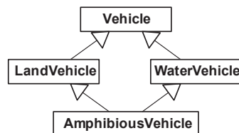
Figure 14.5. A diamond-shaped class hierarchy for amphibious vehicles.
