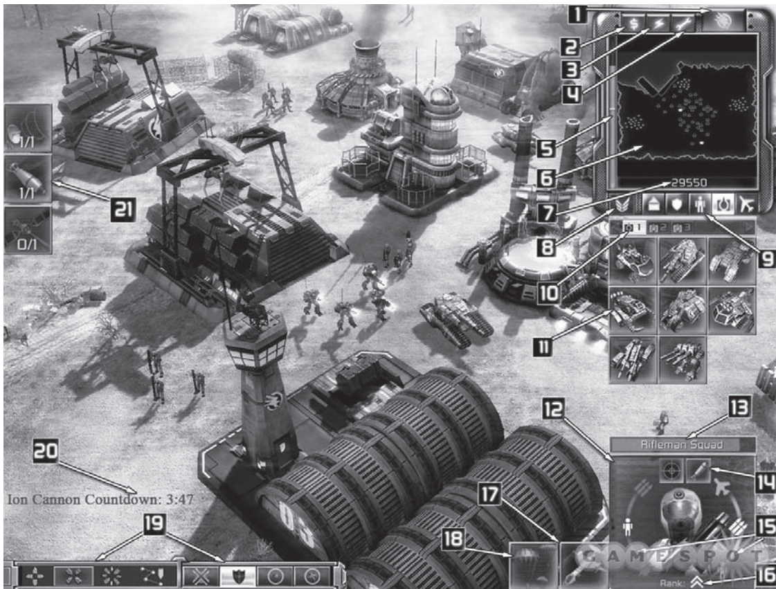
Figure 1.9. Command & Conquer 3 .
