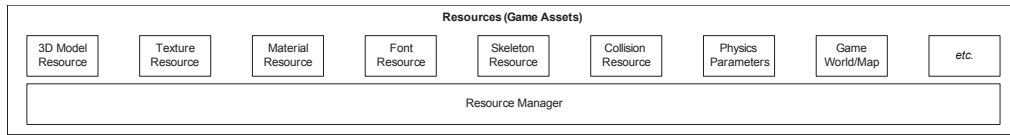
Figure 1.18. Resource manager.
