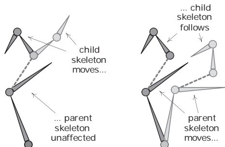
Figure II.60. An attachment, showing how movement of the parent automatically produces movement of the child but not vice-versa.
