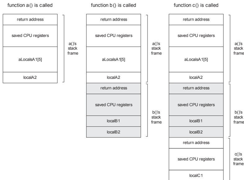
Figure 3.10. Stack frames.
