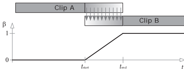
Figure II.27. A smooth transition, in which the local clocks of both clips keep running during the transition.
